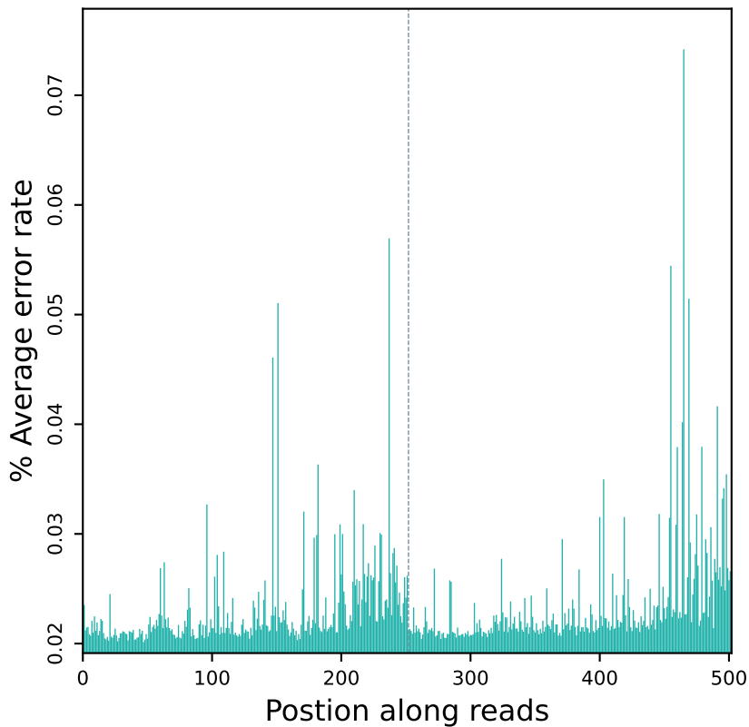
Error rate distribution along reads (R10205)
